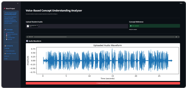
Figure 6: Audio Upload
