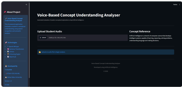
Figure 5: Home Page
