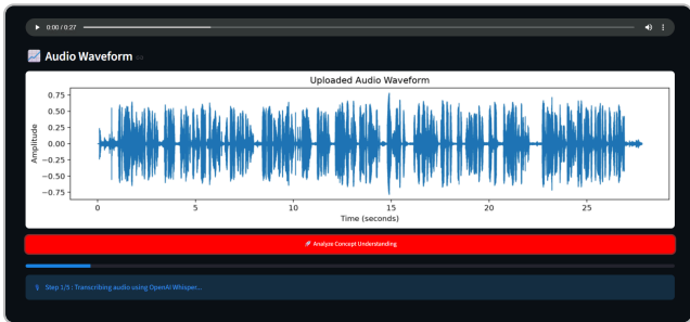
Figure 7: Audio Waveform
